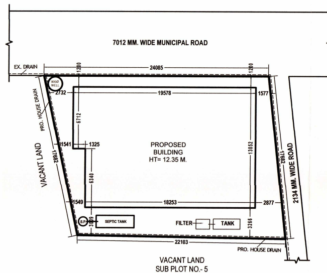
SITEPLAN SCALE- ( 1 : 200 ) DIMENSION ARE IN MM.
