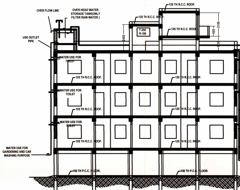
CROSS SECTION OF BUILDING SCALE- ( 1 : 100 )
